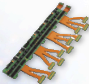
8 Layer Rigid-Flex Assembled
